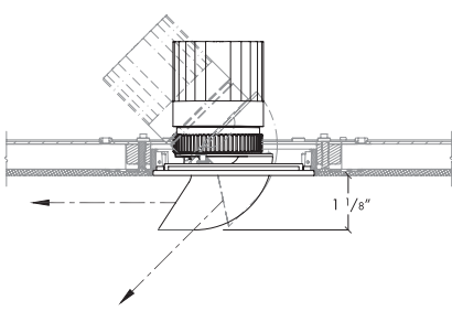
LAMP MODULE M2S - TRIM ASSEMBLY CROSS SECTION DETAIL
