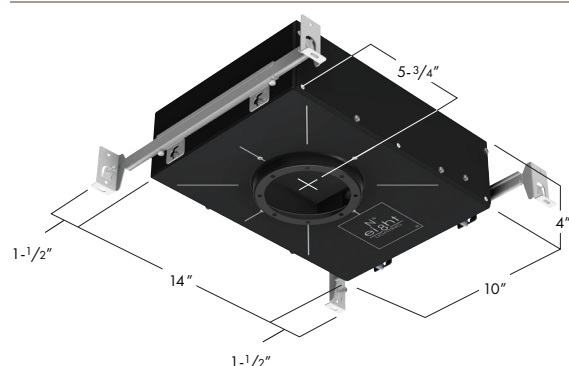
804D-R - LOW PROFILE DEEP CEILING HOUSING - ROUND (Shown with BH mounting accessory)
