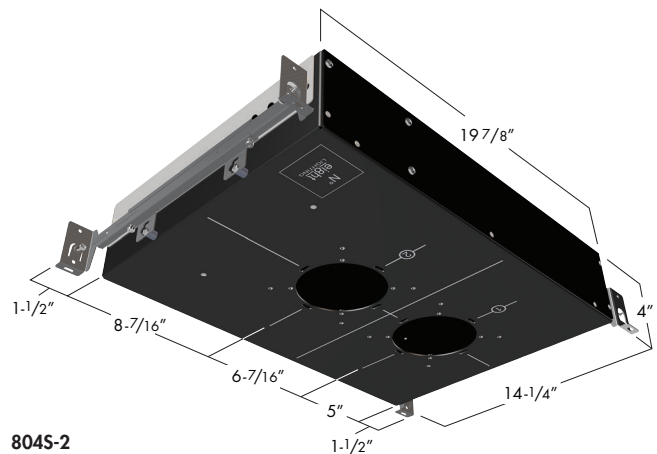
804S-2 LOW PROFILE MULTI-LAMP HOUSING (shown with BH mounting accessory)
