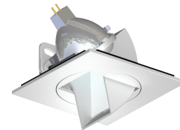
B - MR-16 MIRROR REFLECTOR Use on sloped ceilings for general, accent, and wall wash lighting applications. Features 0-90 degree adjustable aiming angle.
