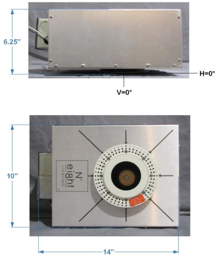
FIG.1 LUMINAIRE
