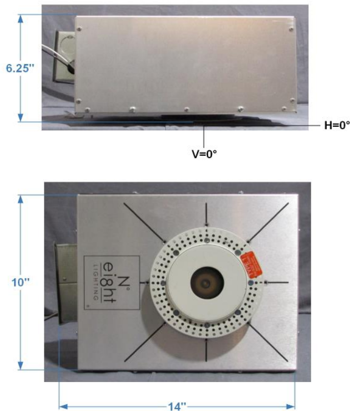
FIG.1 LUMINAIRE
