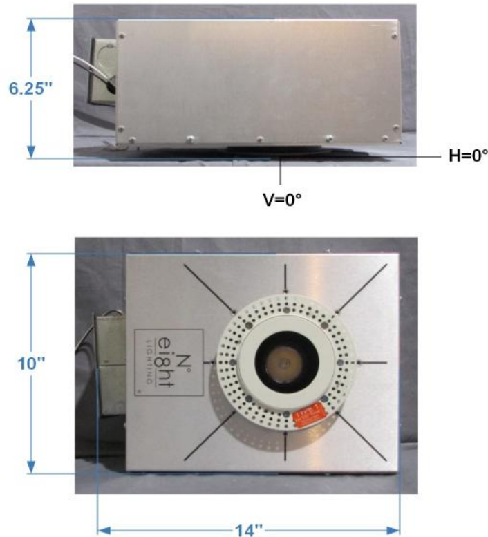
FIG.1 LUMINAIRE
